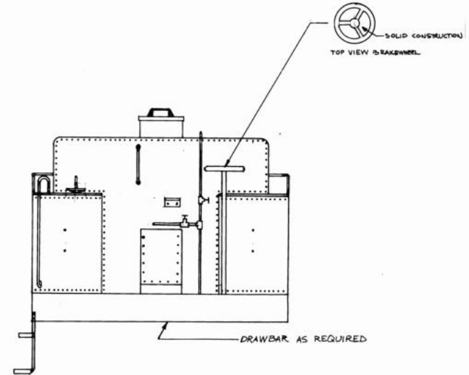
TENDER FRONT VIEW
