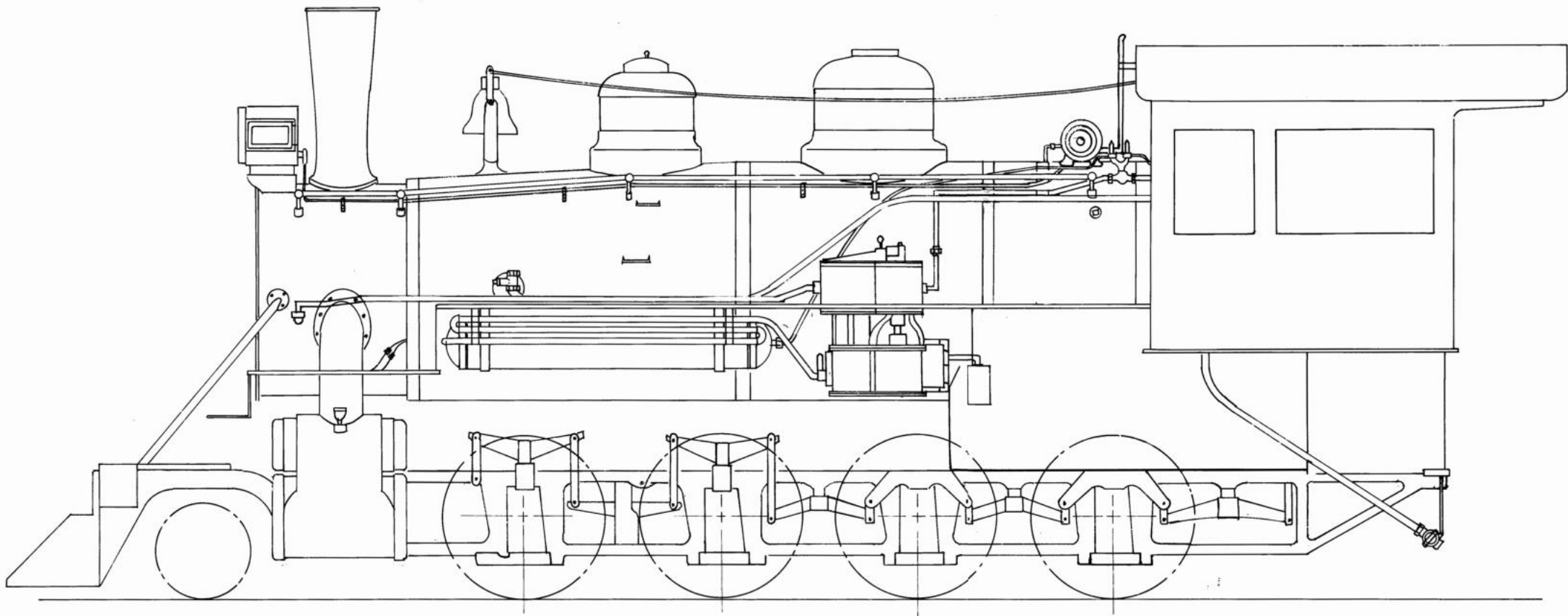
FIREMANS SIDE ELEVATION
