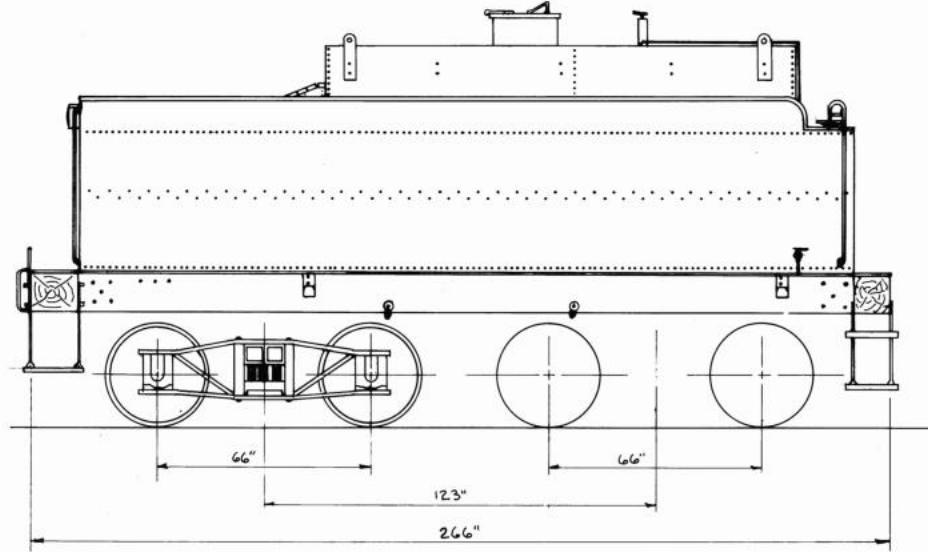
TENDER SIDE ELEVATION
